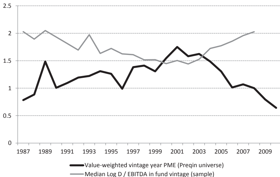
Figure 4. Fund vintage performance and credit spreads. This figure plots the value-weighted vintage year public market equivalent (PME) measure for buyout funds in the Preqin universe against median log net debt to EBITDA for deals in our sample that can be attributed to a certain fund vintage (982 of 1,157 deals satisfy this criterion). Value weighting is by size of funds raised. The benchmark public portfolio used for calculating the PME measure is the CRSP NYSE/Amex/NASDAQ Value-Weighted Market Index. Vintage year refers to the year when the acquiring private equity fund was raised. From the Preqin database, only funds classified as “Buyout” and only funds with complete cash-in–cash-out data are used (648 funds in total).
