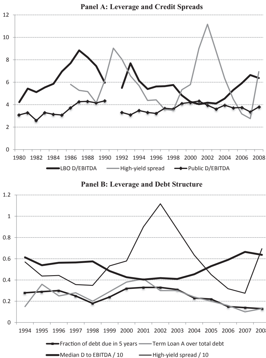
Figure 3. Leverage, credit spreads, and debt structure. This figure presents time-series data on average credit spreads (U.S. high-yield rate minus LIBOR), leverage, and debt structure. Panel A plots credit spreads against median Net Debt to EBITDA for a sample of 1,157 leverage buyout transactions and the corresponding median values for matched public companies. See Table IV for definitions of all variables. Each leveraged buyout is matched to the median value for public firms in the same Fama–French 49 industry, month, and region (United States, Western Europe, Eastern Europe, Asia, or Australia). Panel B plots leverage (divided by 10 for scaling) against debt maturity (measured as the fraction of total LBO debt due in 5 years or less) and the fraction of Term Loan A out of total LBO debt for the deals in our sample between 1994 and 2008.
