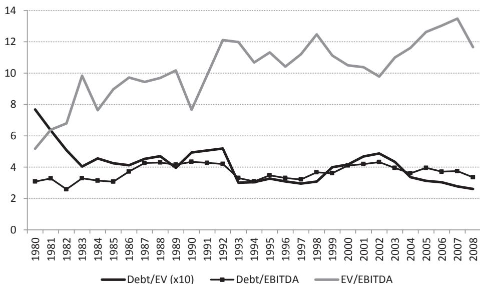
Figure 2. Market trends in leverage and pricing. The figure shows median values of net debt to enterprise value times 10, net debt to EBITDA, and enterprise value to EBITDA for a sample of 1,157 leverage buyout transactions (Panel A) and the corresponding median values for matched public companies (Panel B). Each leveraged buyout is matched to the median value for public firms in the same Fama–French 49 industry, month, and region (United States, Western Europe, Eastern Europe, Asia, or Australia). See Table V for definitions of all variables. There were no buyouts in 1991.
