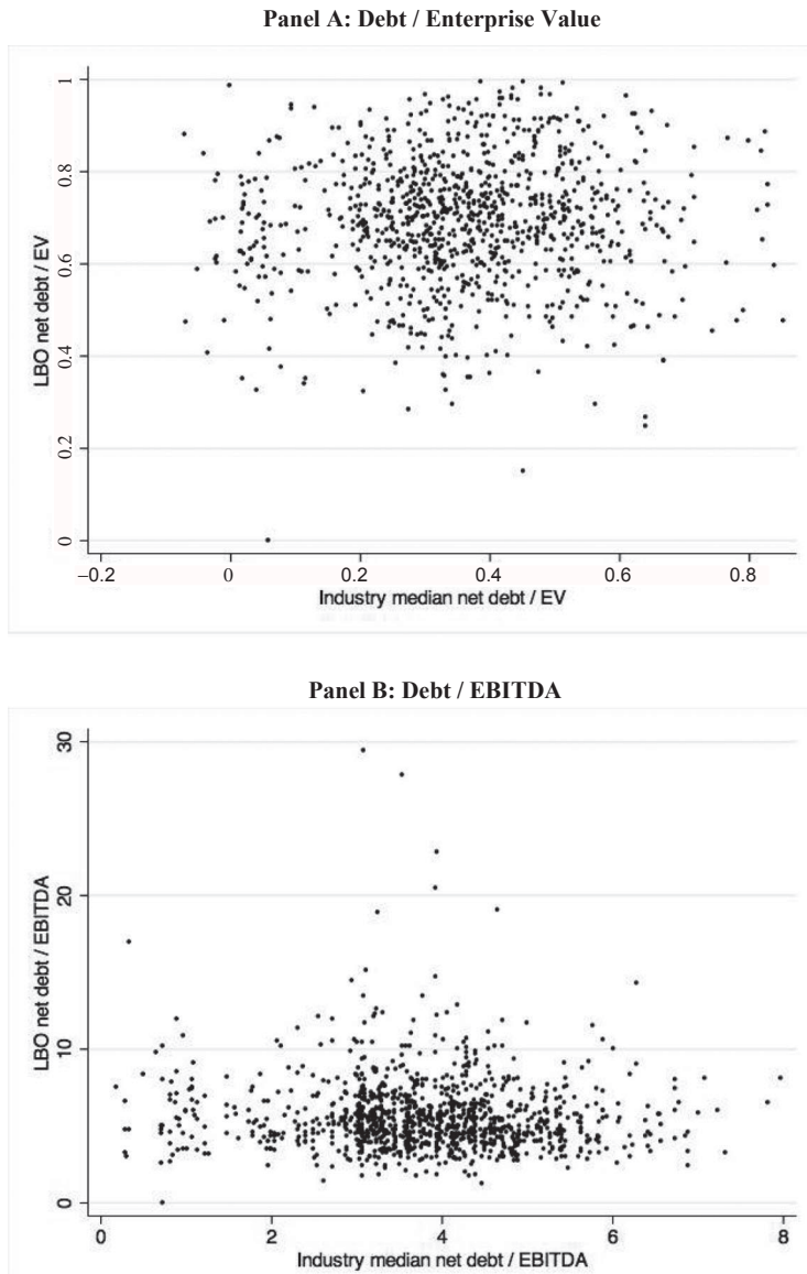
Figure 1. LBO versus public market leverage. This figure shows LBO leverage for the sample plotted against the median public company leverage in the same Fama–French 49 industry, year and month, and region (United States, Western Europe, Eastern Europe, Asia, or Australia) as the LBO. The sample excludes LBOs in the banking and insurance industries (Fama–French industries 45 and 46). In addition, Panel B excludes two LBOs with negative EBITDA at the time of the transaction and the industry median calculation excludes firms with negative EBITDA. Leverage is measured as net debt to enterprise value (market value of equity plus debt minus cash and short-term investments) in Panel A, and net debt (i.e., debt minus cash and short-term investments) to EBITDA in Panel B. For public companies, net debt to EV is calculated using equity market value in the month preceding the date of the closing of the syndicated loan for the corresponding LBO. For the LBOs, net debt does not include contingent debt such as lines of credit.
